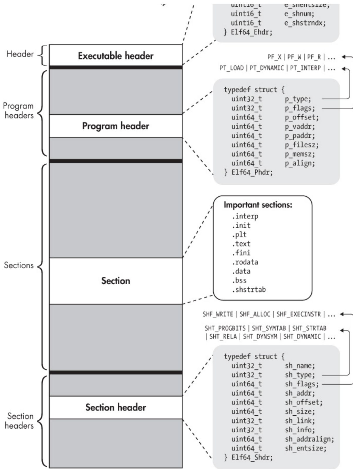
Figure 2-1: A 64-bit ELF binary at a glance
