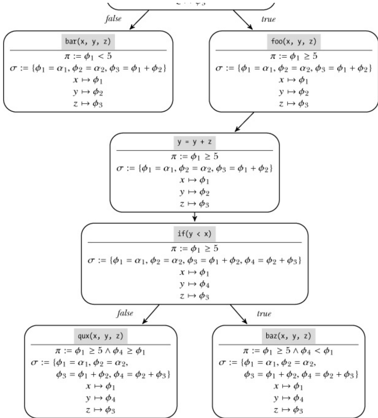
Figure 12-1: Path constraints and symbolic state for all paths in the example function
