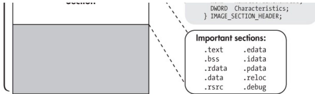
Figure 3-1: A PE32+ binary at a glance
