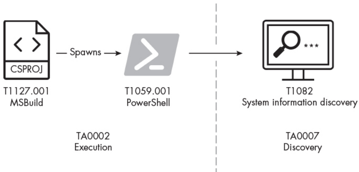
Figure 8-1: The initial stages of the emulation scenario
