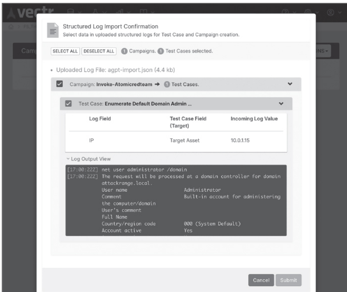
Figure 8-2: The imported ATTiRe log
