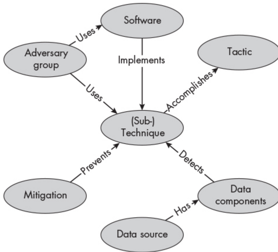
Figure 2-2: Relationships among the object types in ATT&CK
