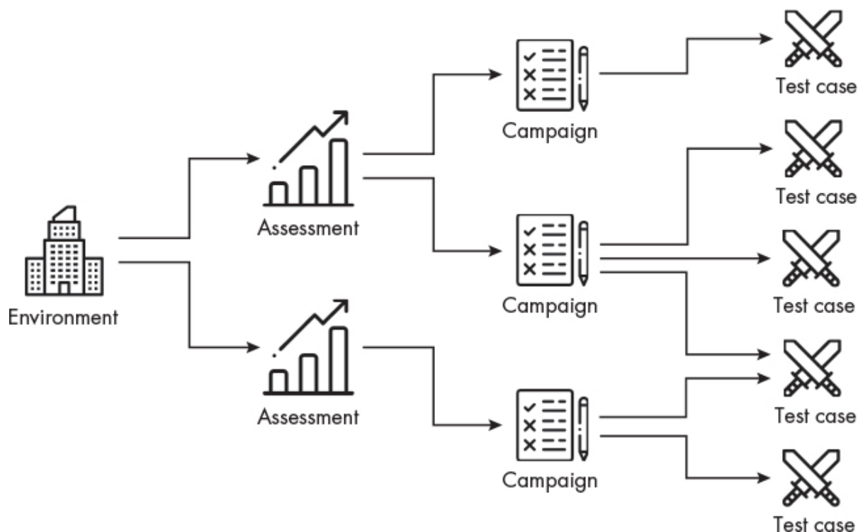
Figure 11-4: The nested structure of VECTR environments
