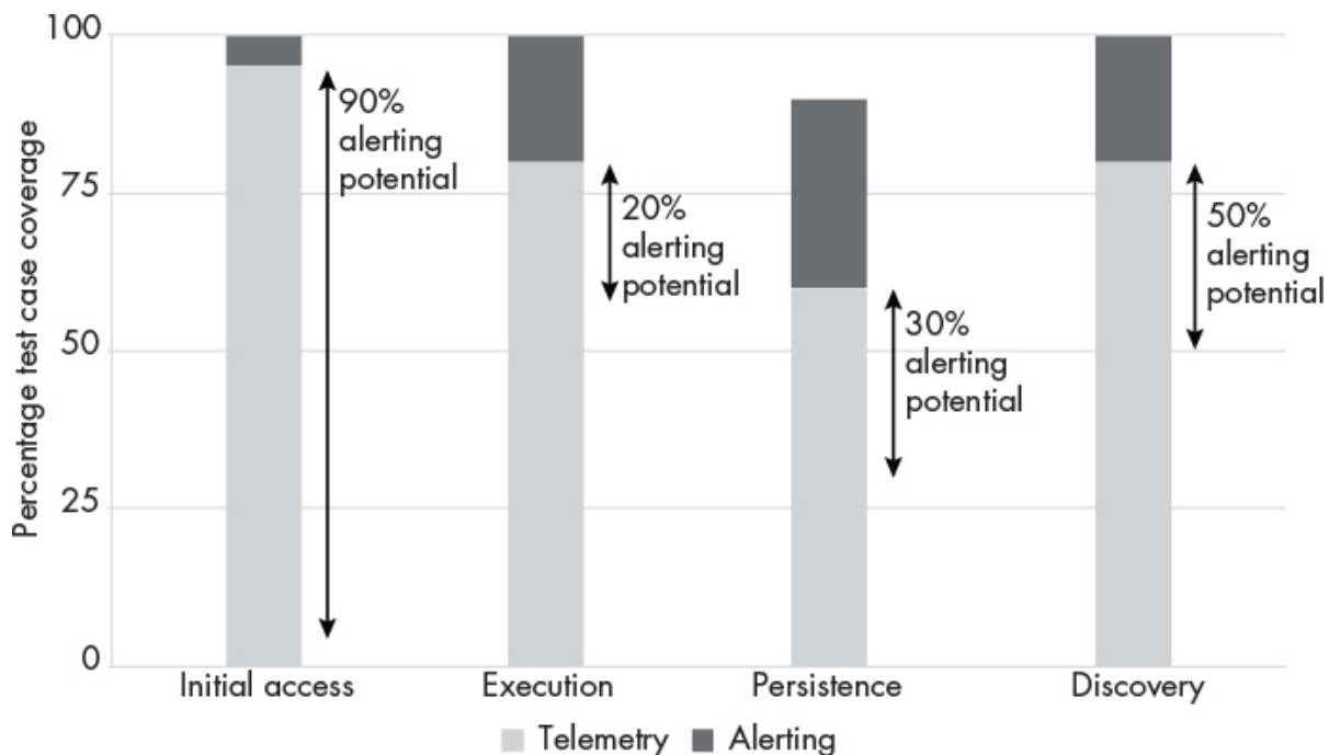
Figure 3-6: Capturing the alerting potential
