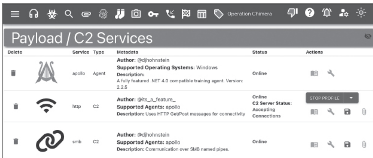
Figure 10-2: Installed agents and C2 profiles
