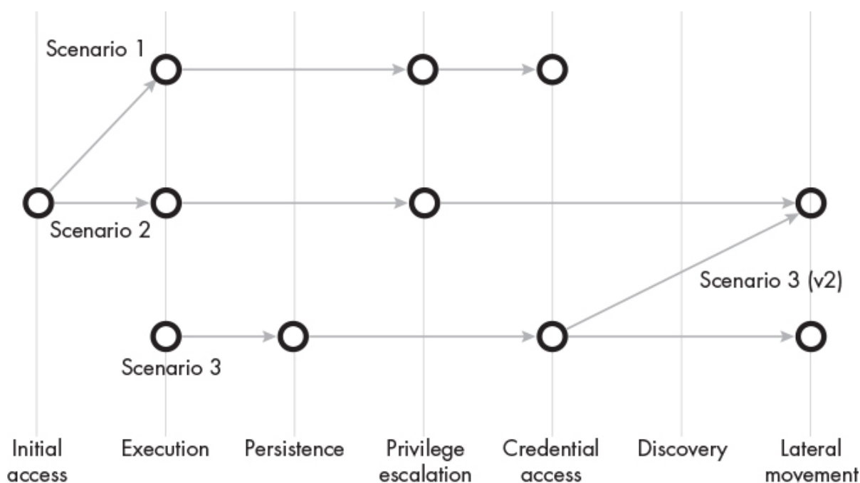
Figure 4-1: Plotting attack-chain scenarios
