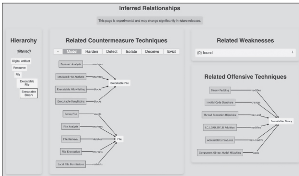
Figure 2-6: The object relationships for an executable binary
