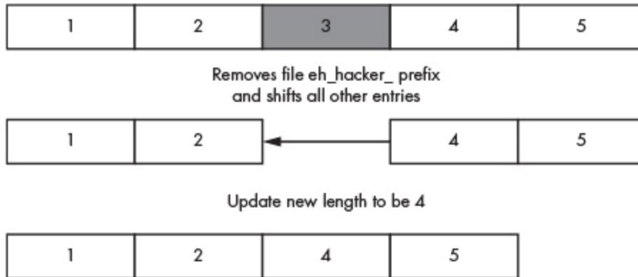
Figure 11-5: How the directory entry array is modified
