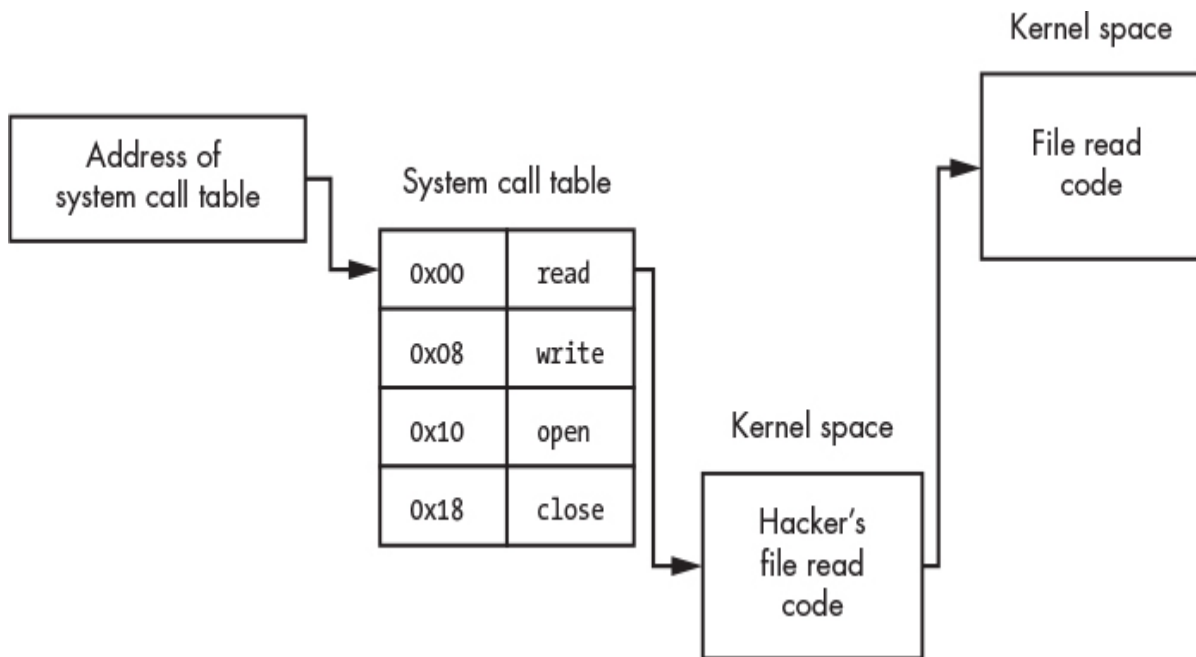
Figure 11-4: An overview of the hooking process
