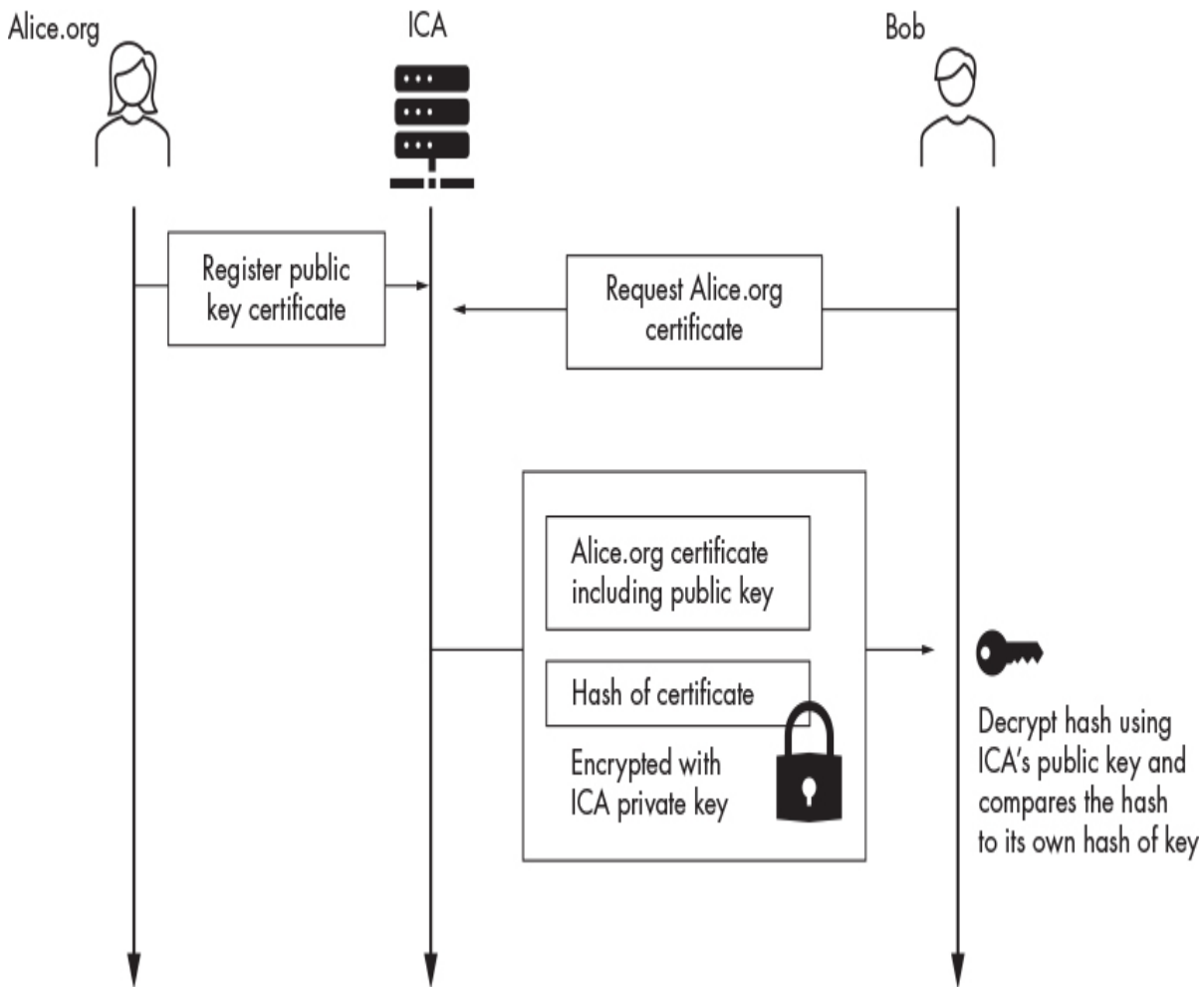
Figure 6-4: An overview of the certificate validation process
