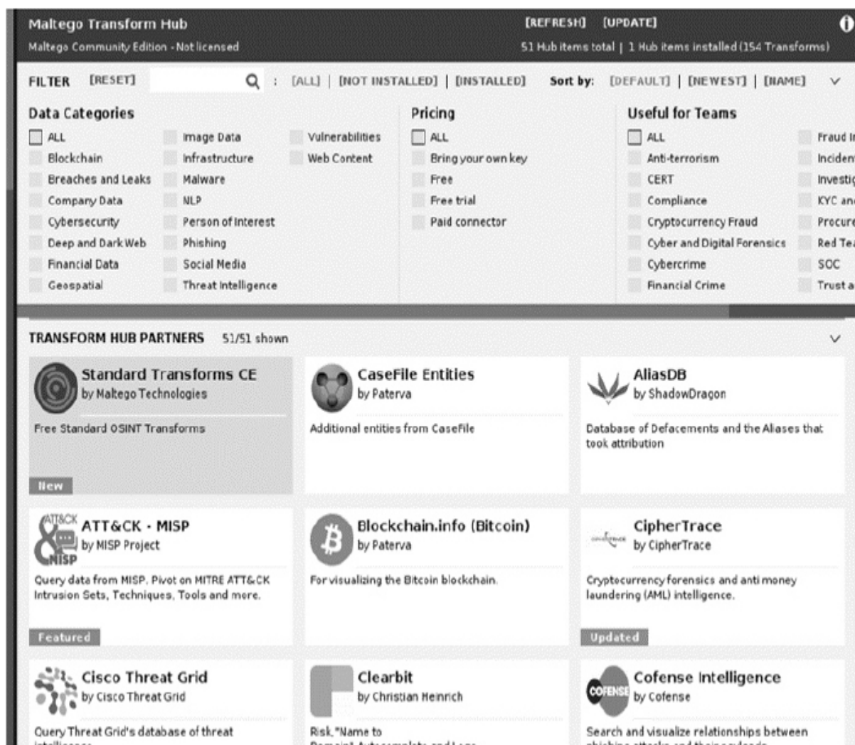
Figure 8-5: The Transform Hub's list of transforms
