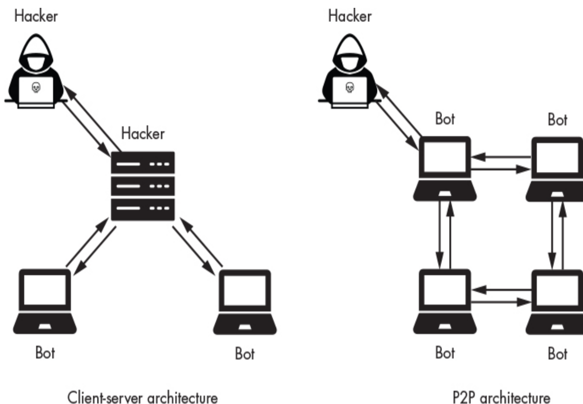
Figure 4-7: Two botnet architectures: client-server and P2P
