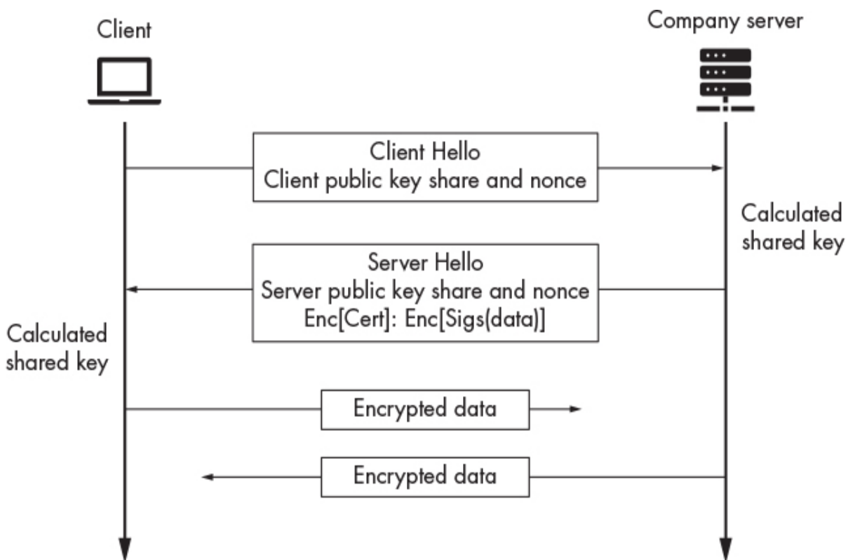
Figure 6-1: The TLS message exchange
