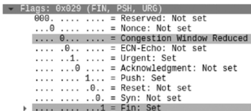
Figure 4-6: An XMas scan
