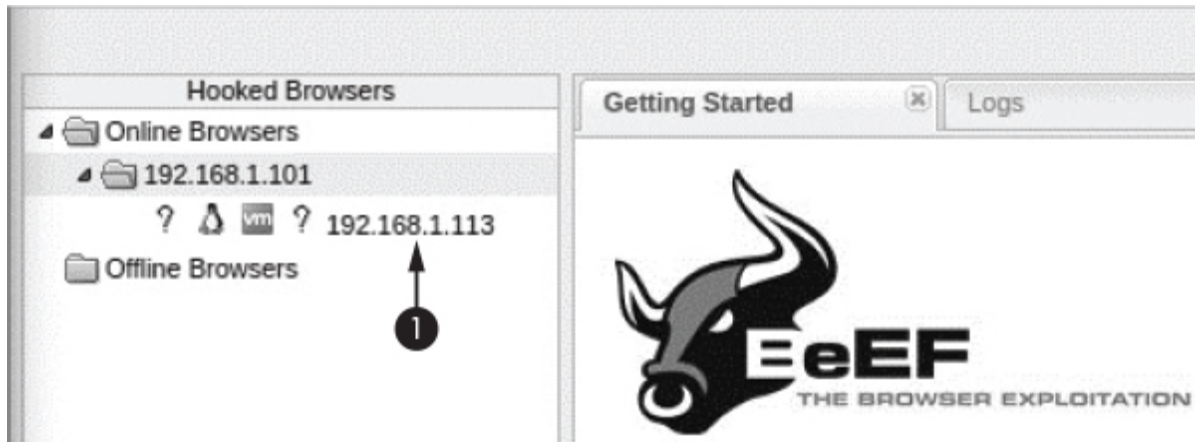
Figure 13-10: List of browsers running the malicious JavaScript
