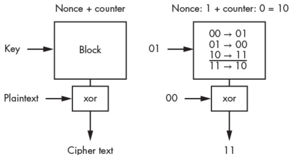
Figure 5-6: The design of the CTR
