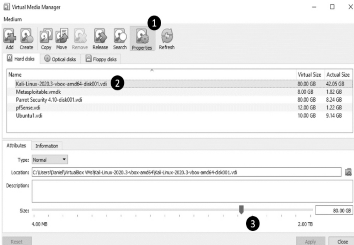
Figure 8-6: How to increase hard drive size
