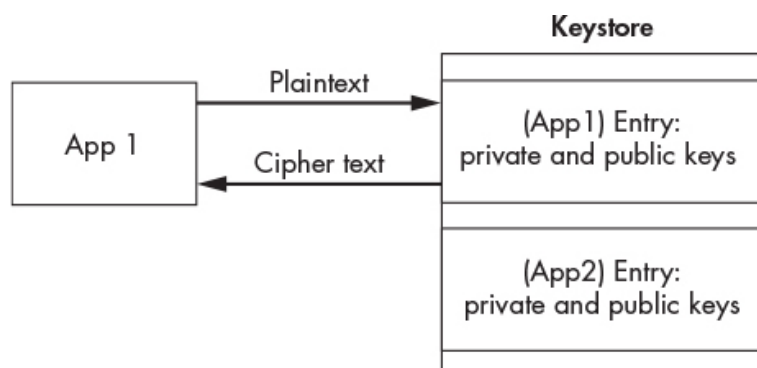
Figure 10-10: Key material never leaves the Keystore.
