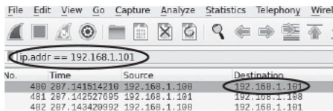
Figure 3-9: Filtering packets in Wireshark
