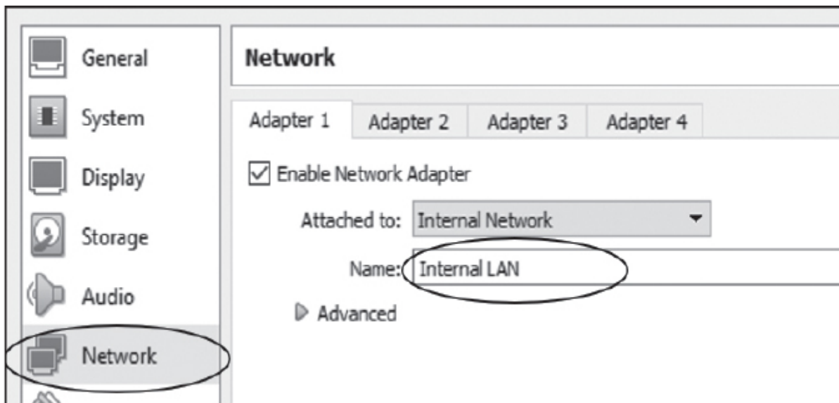
Figure 1-10: Configuring the Metasploitable internal network
