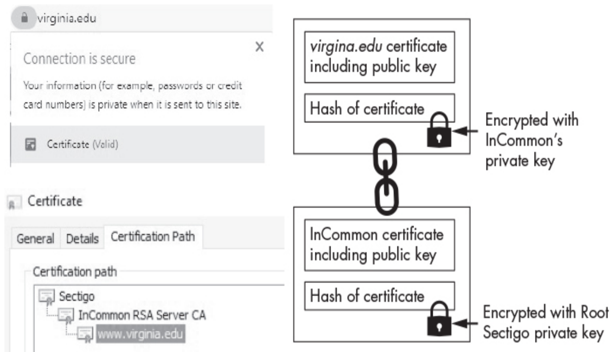
Figure 6-5: The path of official certificates
