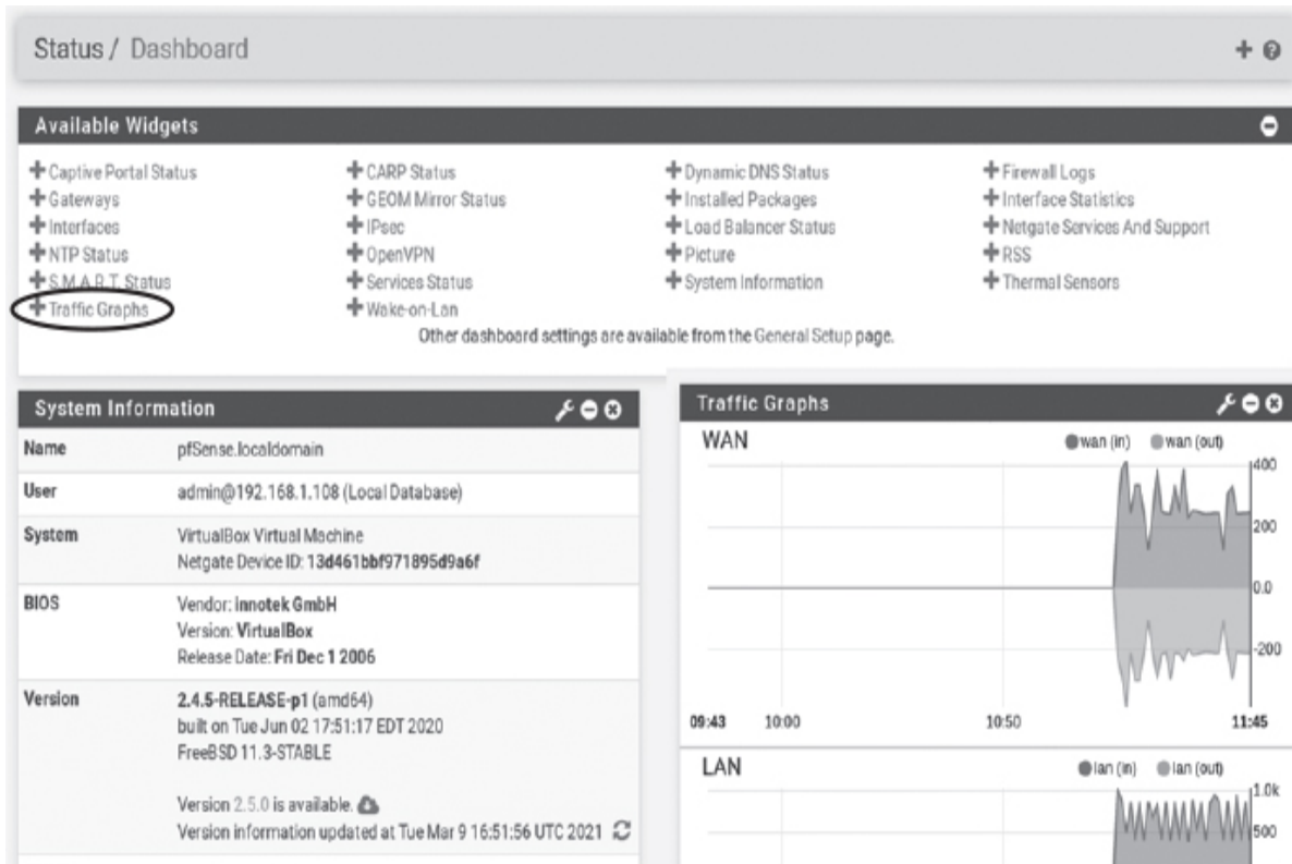
Figure 3-14: The pfSense dashboard
