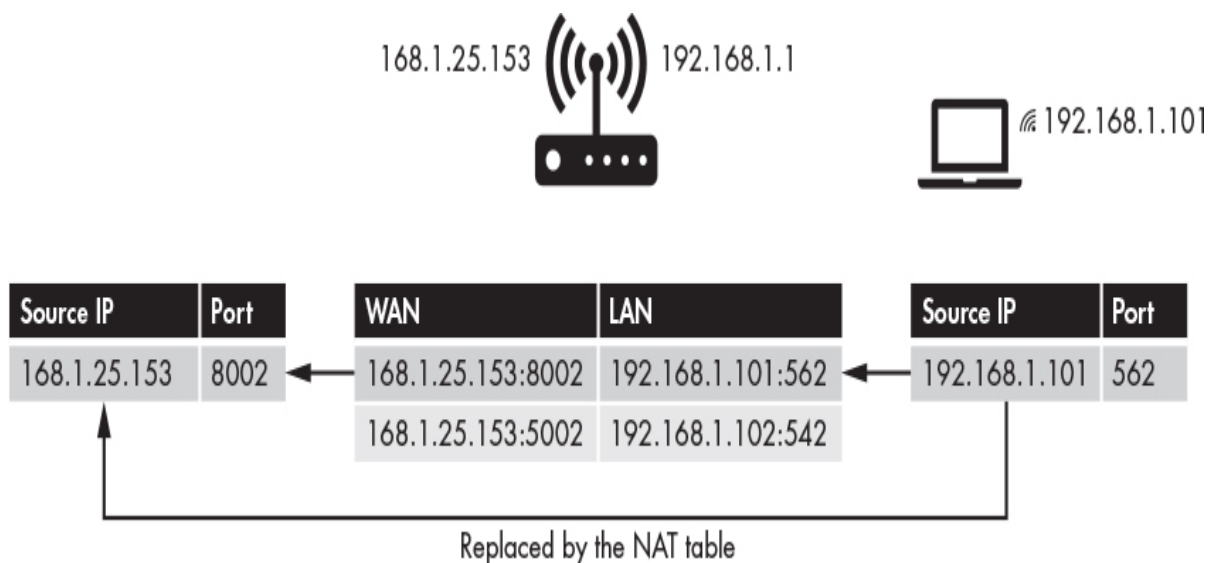
Figure 8-9: How the source IP address and port are replaced
