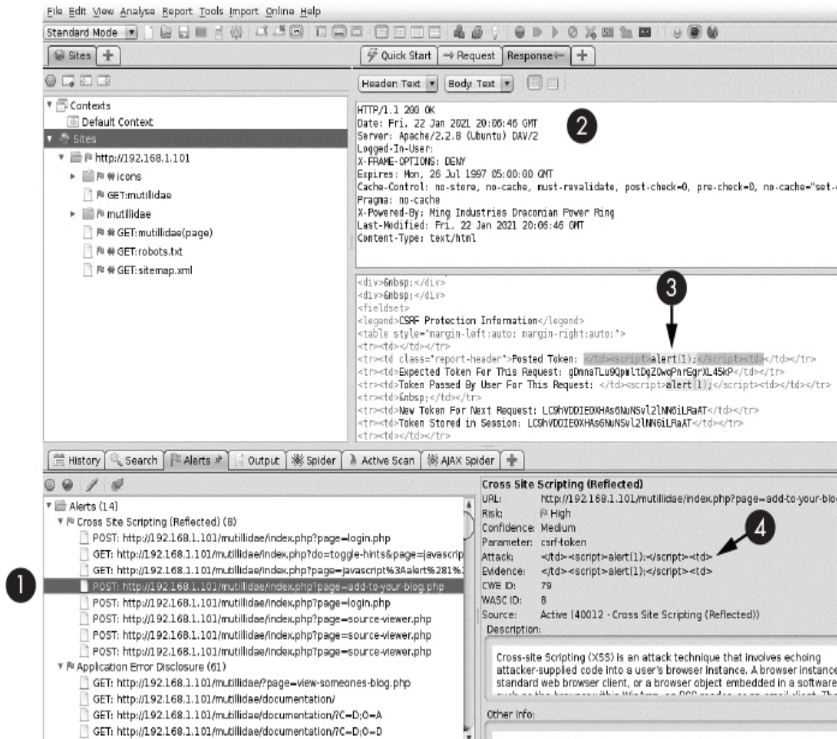
Figure 13-8: The result of running a quick ZAP scan
